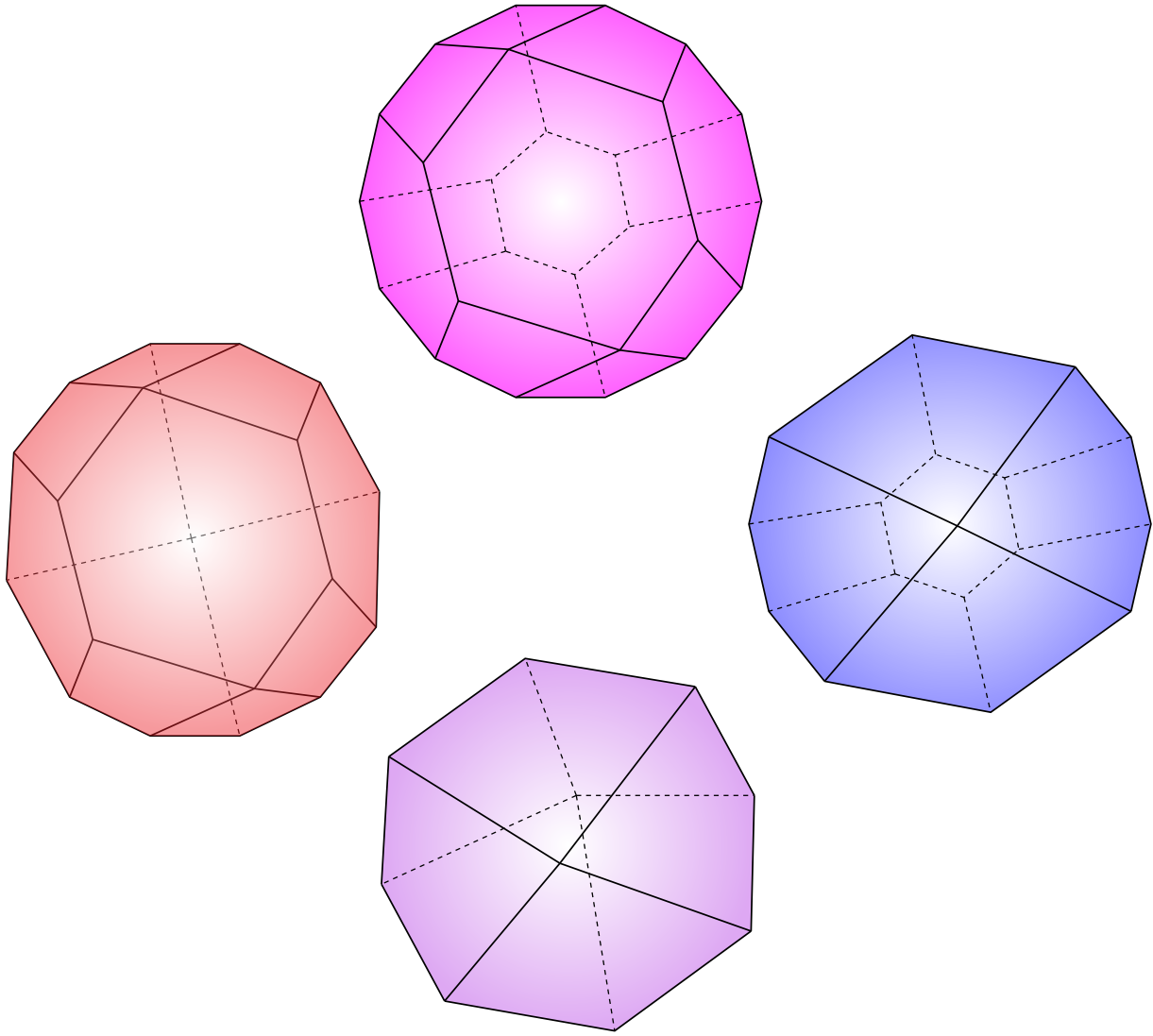
Figure 19: Top: the multiplihedron for the acyclonestohedron of the four-element diamond poset. On the left is the domain quotient, on the right the range quotient, and at the bottom is the interval polytope of the order polytope of the diamond. Note that this interval polytope of the order polytope is a trapezohedron, with a side view in Figure 18. It turns out to be the same polytope as for the bowtie poset, as seen in Figure 1.
