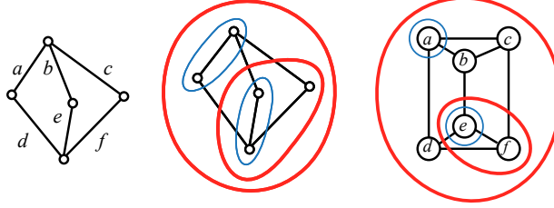
Figure 6: A colored piping on the poset with Hasse diagram at left, and its induced colored tubing on the line graph of that Hasse diagram, on the right. Some facet tubings induced by pipings that contain this piping are shown in Figure 3, and several maximal tubings with coordinates calculated are shown in Figure 13.
