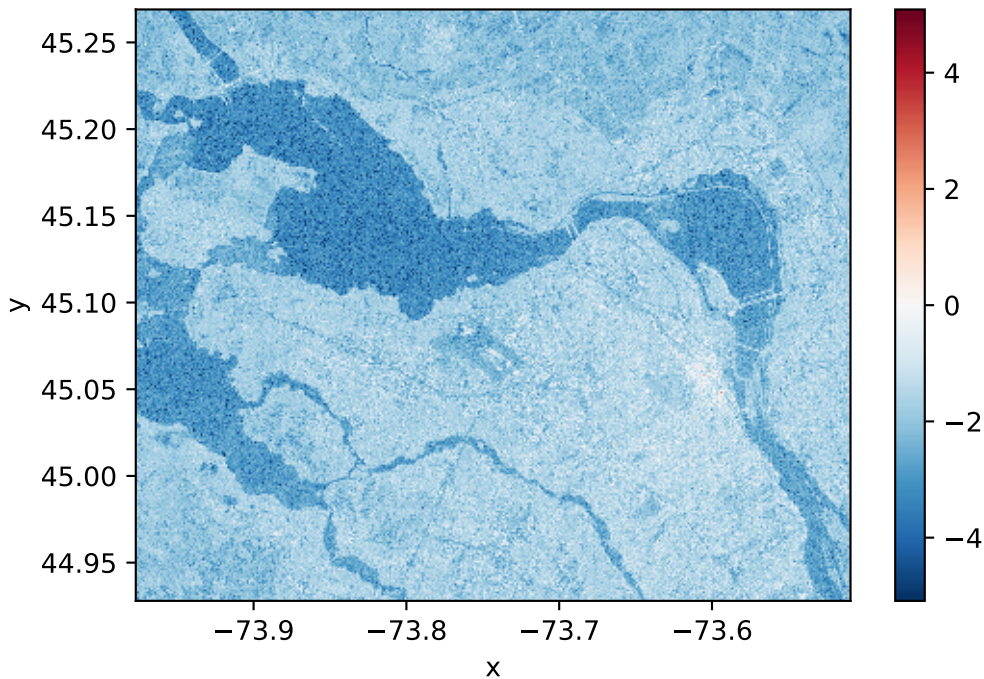
Image SAR Sentinel-1 (dB)
