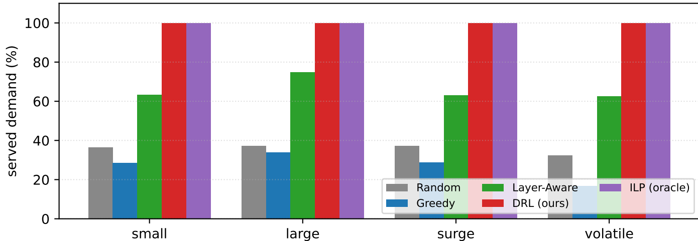
QoS coverage of (user, service) demand
