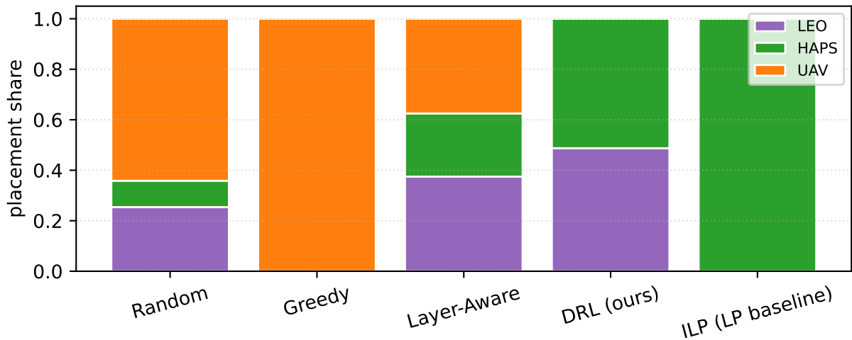
Per-layer share of microservice placements (small scenario)
