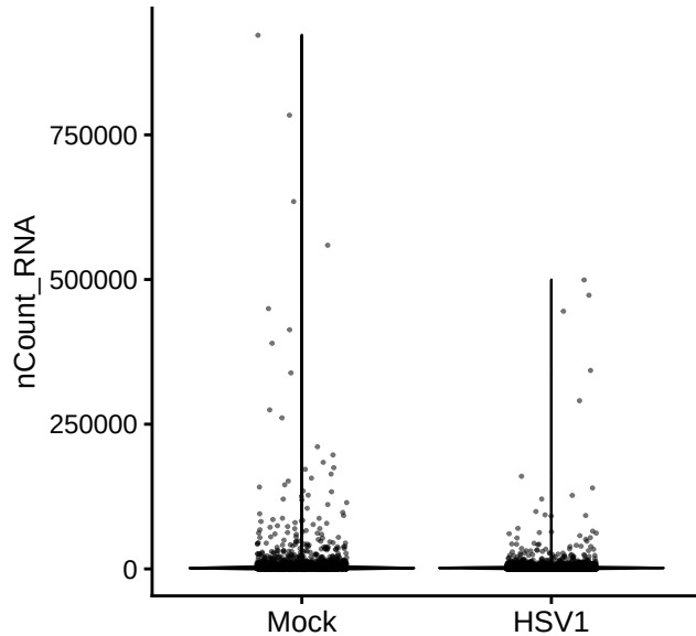
nCount_RNA
