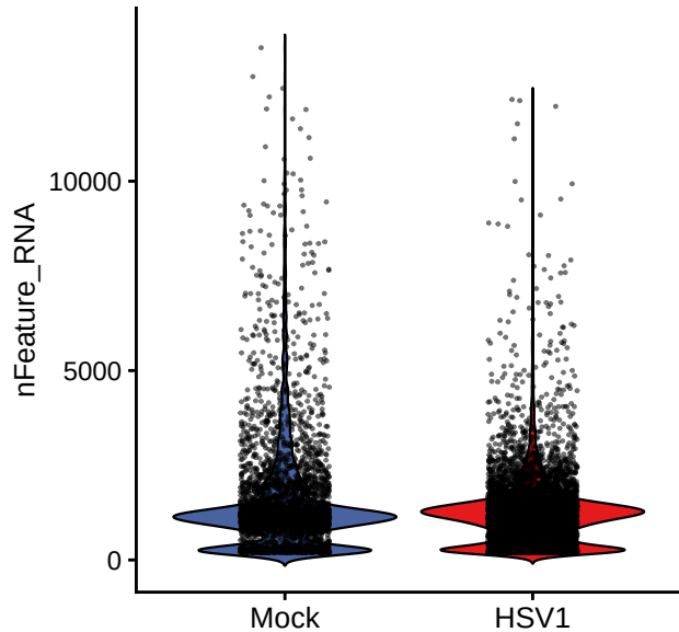
nFeature_RNA
