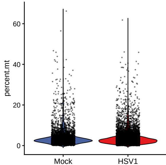
percent.mt
