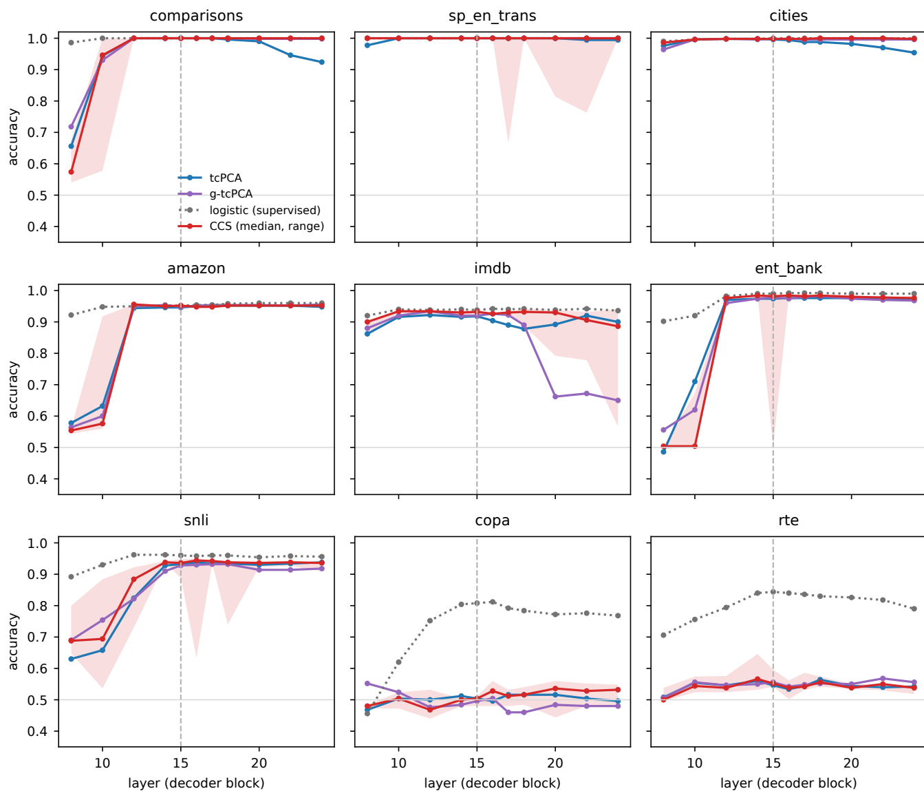
llama3_8b - period token (dashed: block 15, used in the paper)
