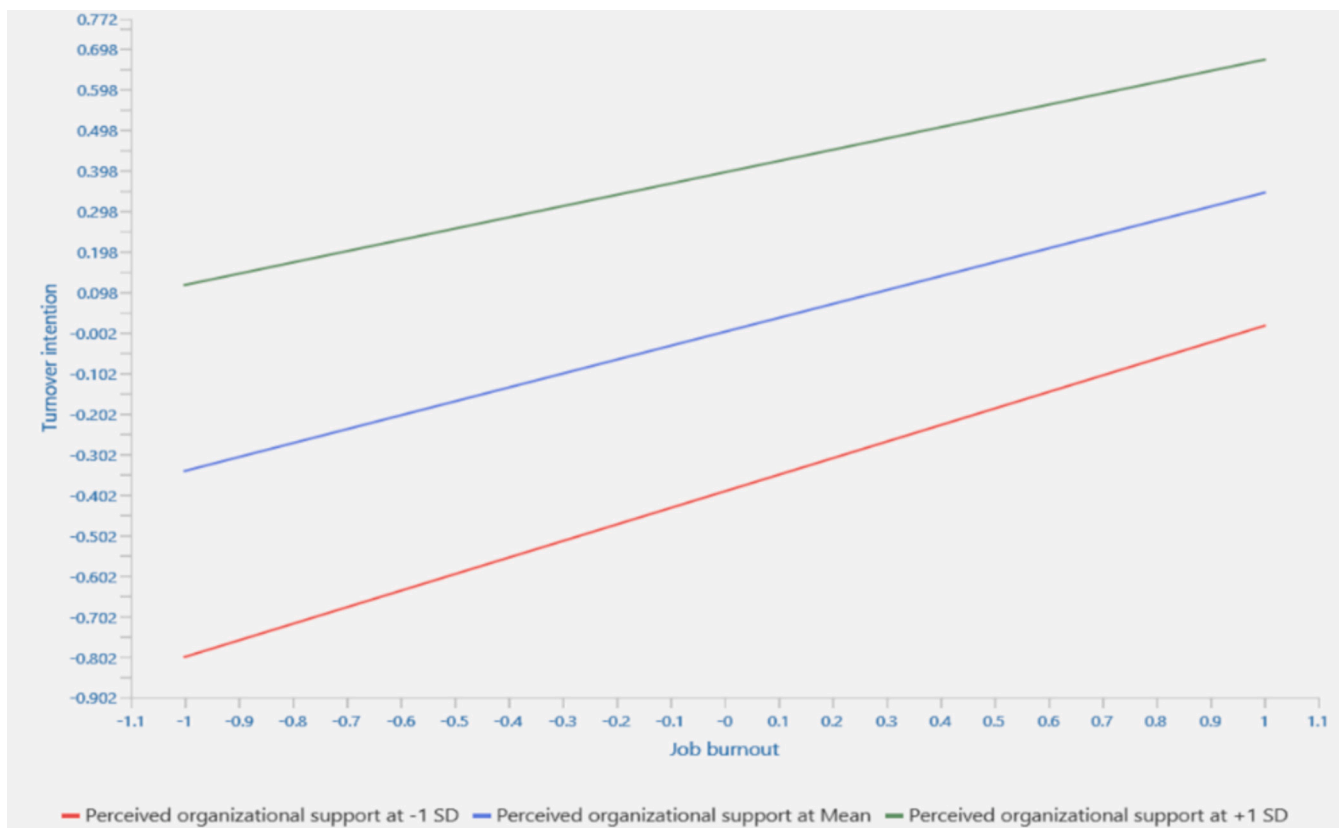
Fig. 4. POS dampened the positive association between JB and TI.
