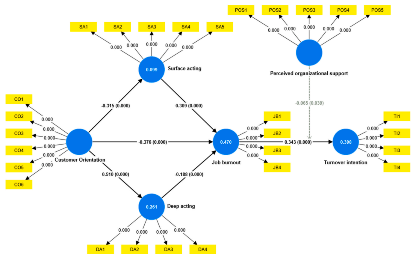
Fig. 3. The structural model.
