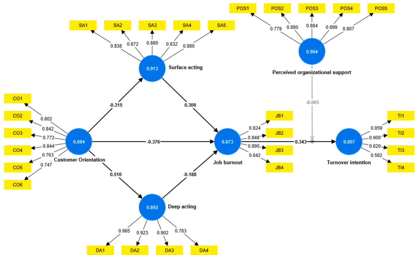
Fig. 2. The measurement model.
