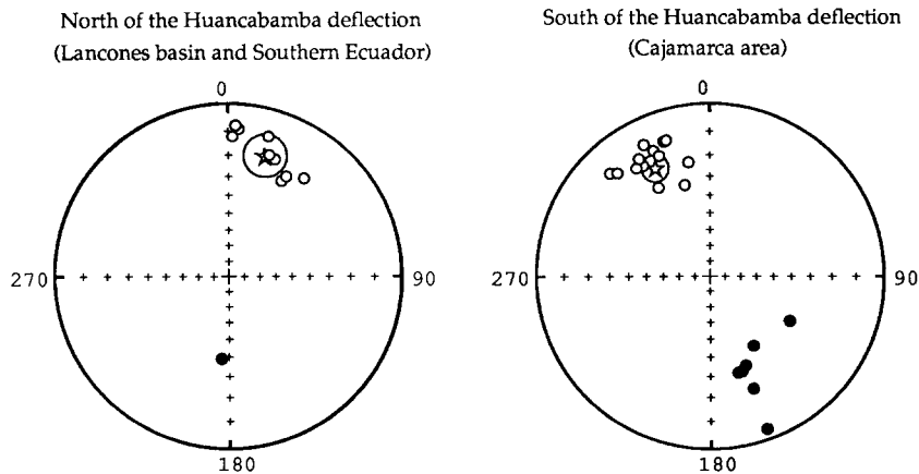
Fig. 4. Equal area stereographic projection of the mean direction of paleomagnetic vectors for the sampled formations on both sides of the Huancabamba deflection. Open circles correspond to upper-hemisphere and full circles to lower-hemisphere projections. Big circles correspond to the 95% confidence area about the mean (stars).
