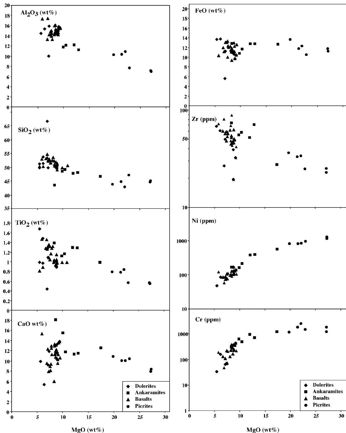
Fig. 4. Al 2 O 3 (wt.%), SiO 2 (wt.%), TiO 2 (wt.%), CaO (wt.%), FeO (wt.%), Zr (ppm), Ni (ppm), and Cr (ppm) vs. MgO (wt.%) correlation diagrams of dolerites, ankaramites, basalts and picrites.
