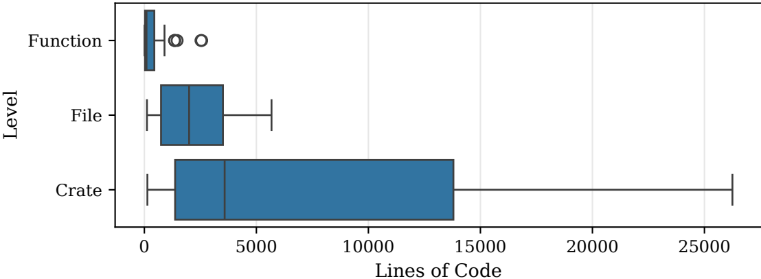
Code Variant Size Distribution by Level
