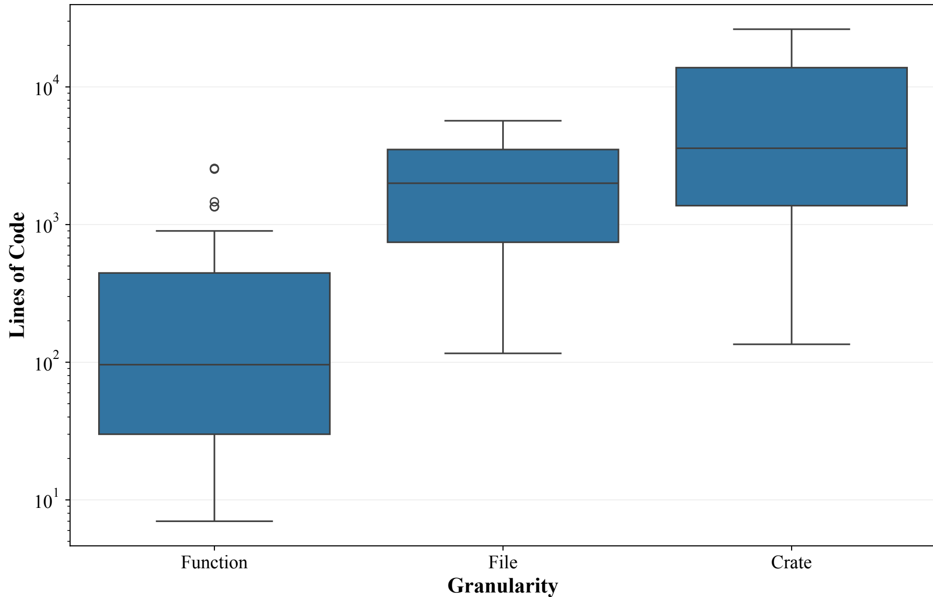
Code Sample Size Distribution by Granularity
