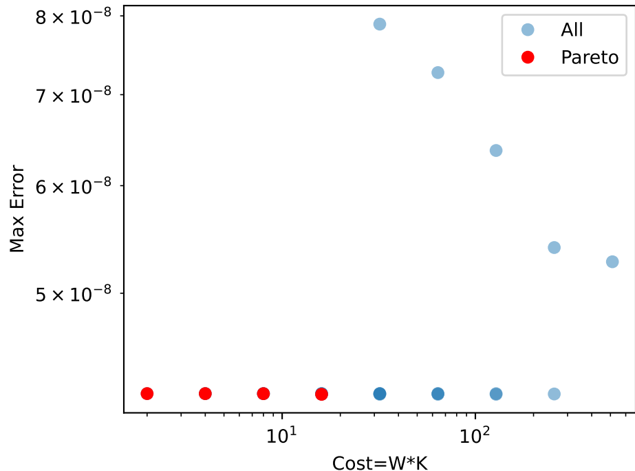
Error vs Cost
