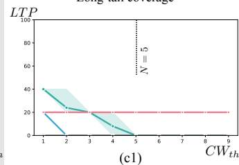
Long-tail coverage
