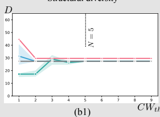
Structural diversity
