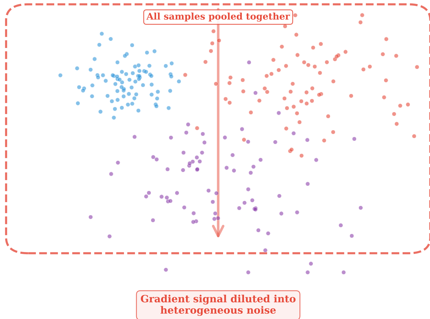
Figure 1. CAGate mechanism: (a) NOTEARS pools all samples, diluting gradient into noise; (b) CAGate partitions samples and applies MAD-aware gating.
