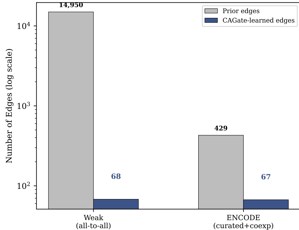
(a) Edge Counts: Prior vs Learned
