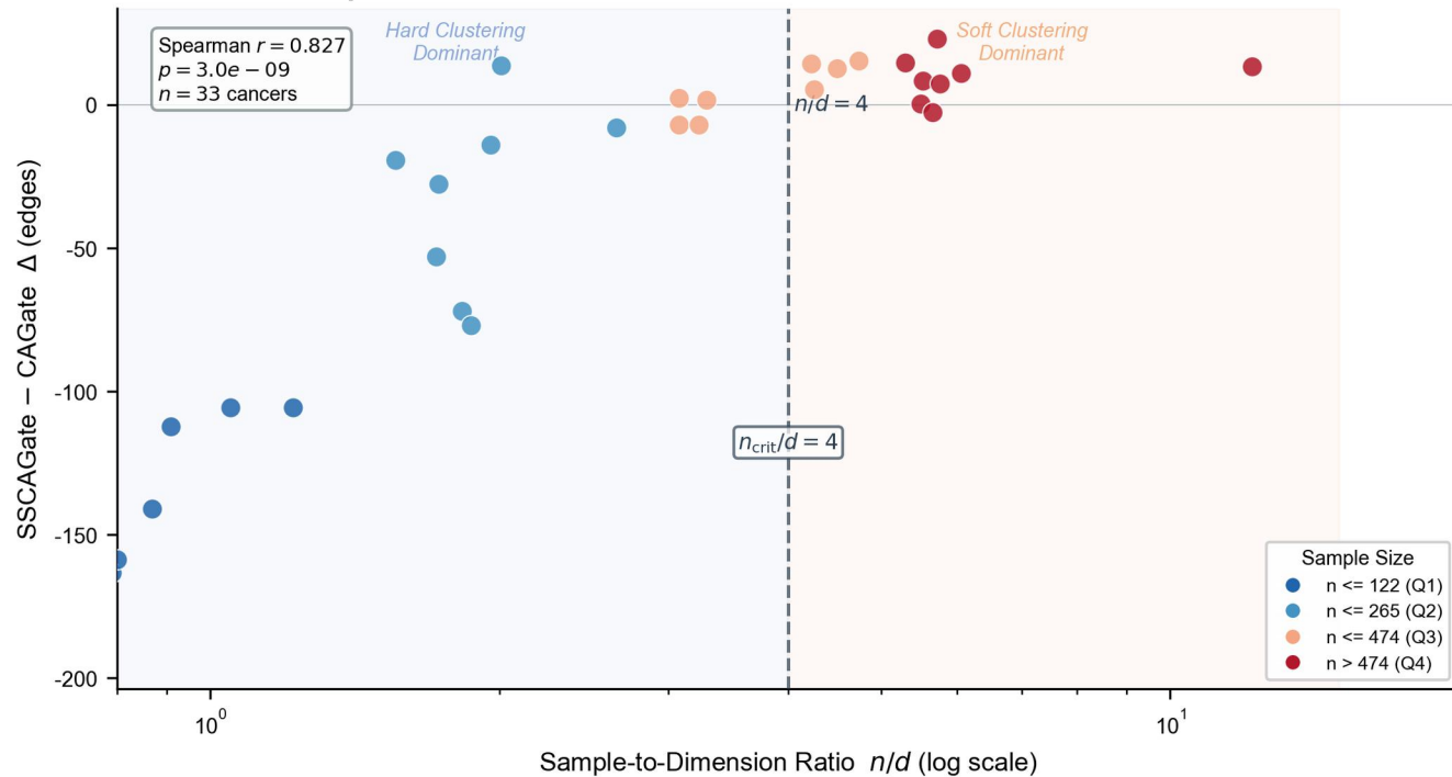
a Universal Sample-Size Phase Transition
