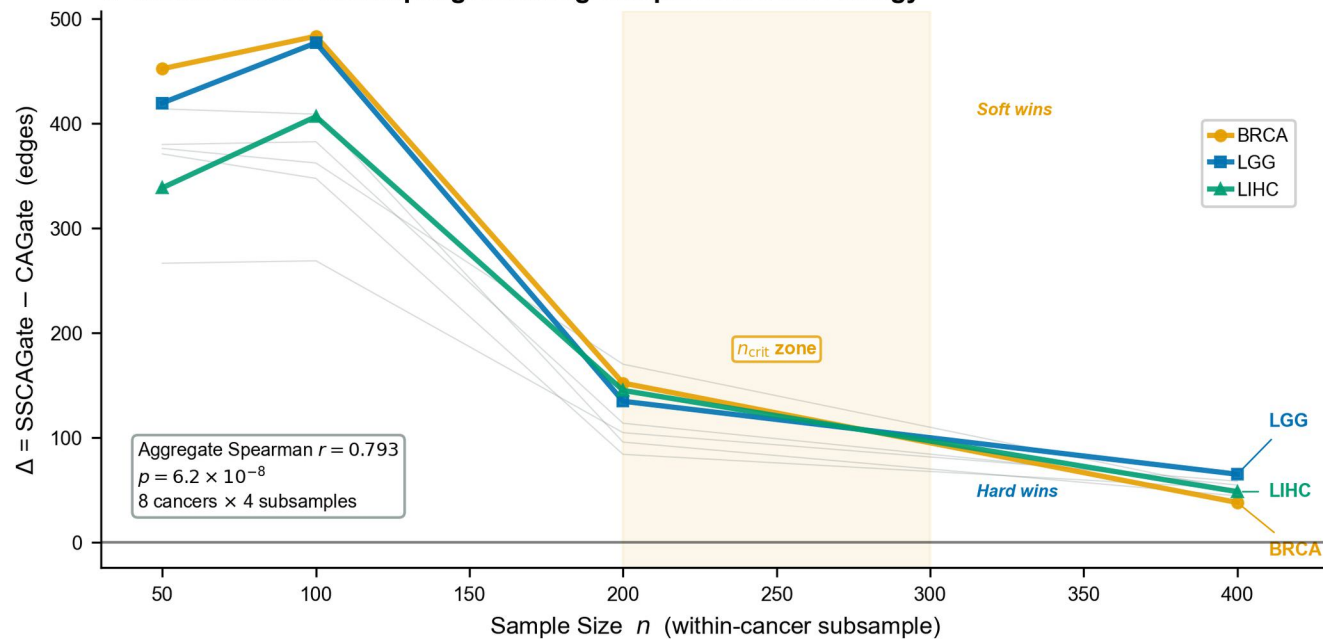
b Within-Cancer Resampling: Isolating Sample Size from Biology
