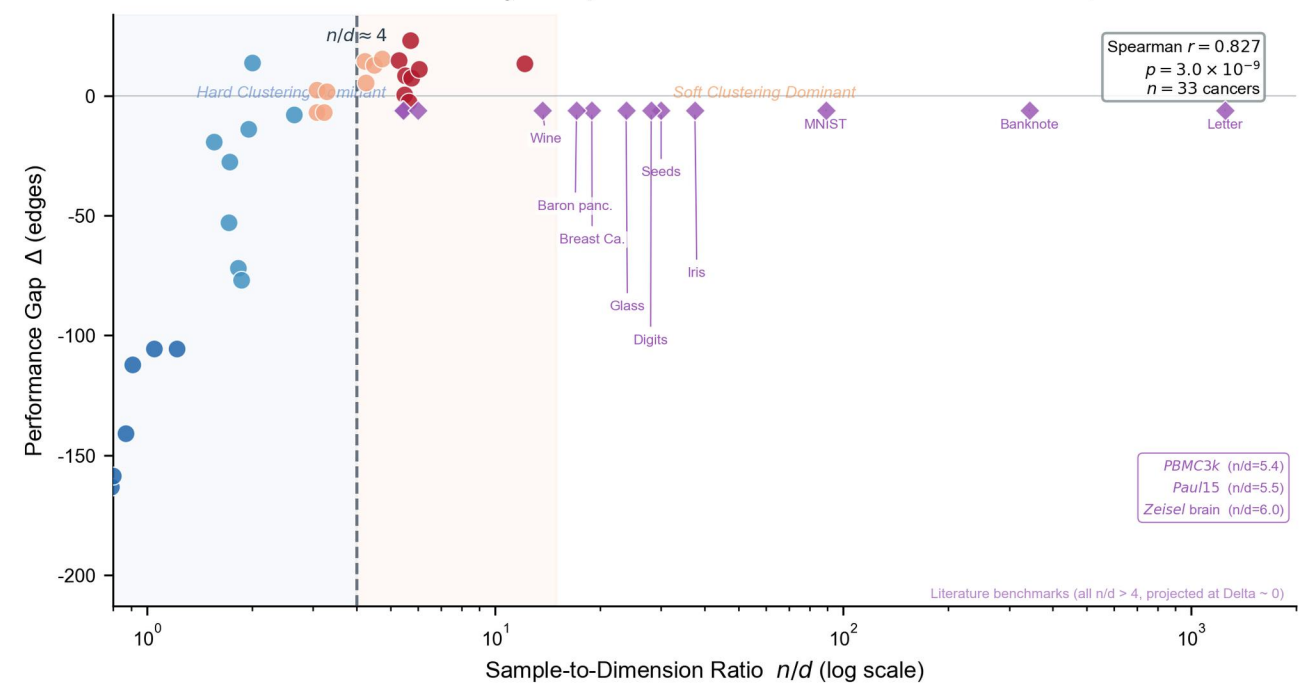
d Literature Benchmarks Overlay: Independent Benchmarks Confirm the Same n/d Threshold
