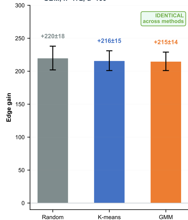
c | Clustering comparison - METHOD INVARIANT GBM, n=172, d=100
