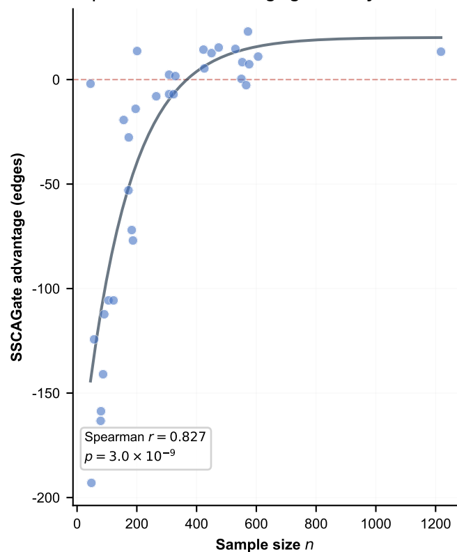
a | Phase transition: edge gain decays with n
