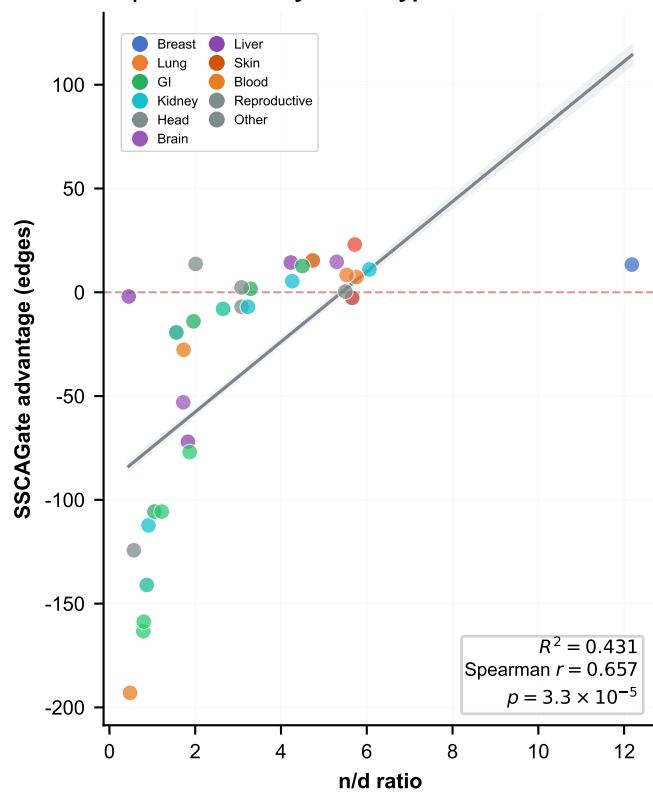
b | n/d scatter by tissue type - structured residuals
