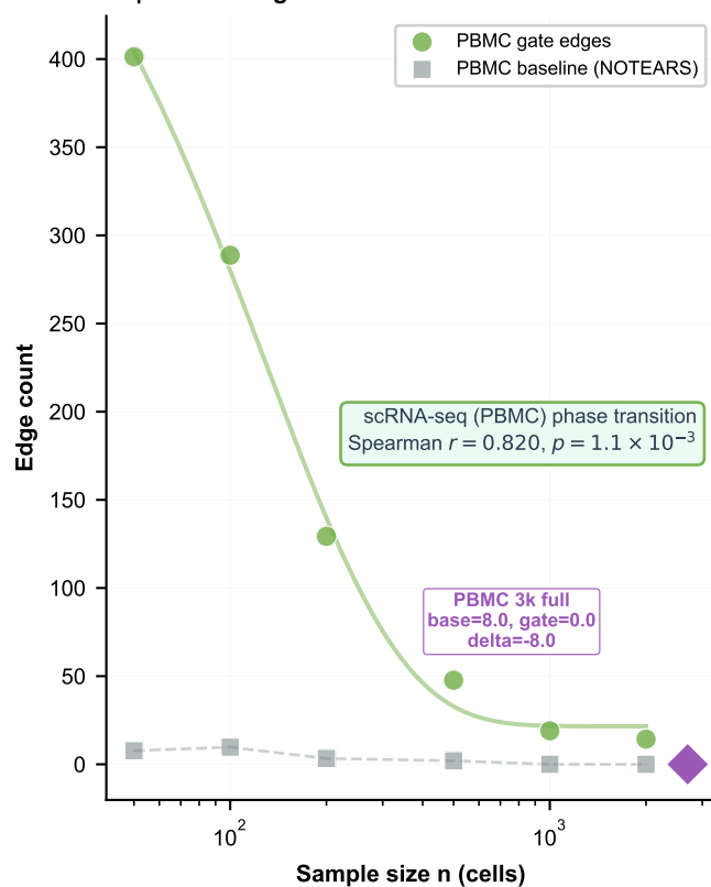
d | PBMC single-cell validation - real benchmark data
