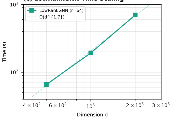
(c) LowRankGNN Time Scaling
