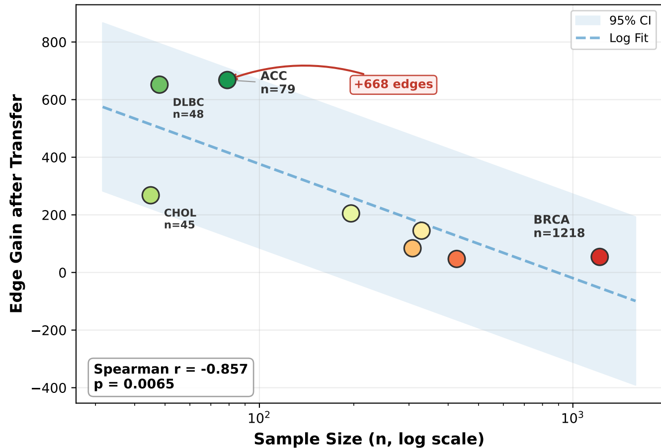
(a) Zero-Shot Transfer: Small-Sample Amplification
