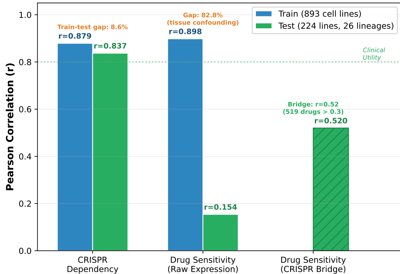
(b) Prospective Validation: 80/20 Stratified Split
