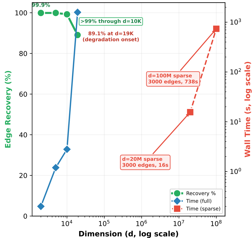
(a) Extreme Scale (d=2K to 100M)
