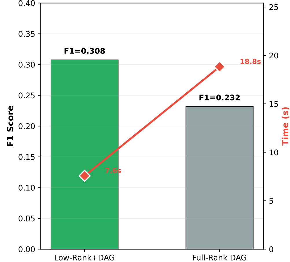
(c) Sachs: DAG Constraint Benefit (d=11, n=7466)
