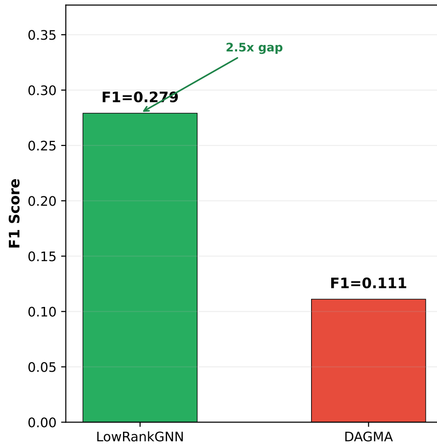
(b) Cross-Domain: Financial Panel (d=30, n=500)
