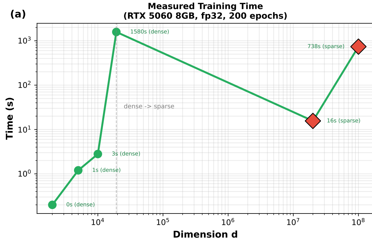
Figure A1: Extreme-Scale Training Dynamics ( 10^4 to 10^8 Variables)
