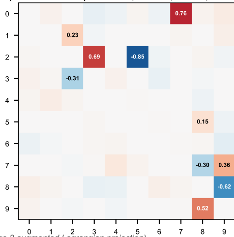
d) Deviation D1 (rewired 2,5=-0.85, new 0,7=+0.76)
