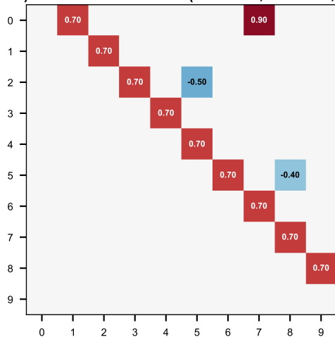
b) Ground truth Batch 1 (rewired 2,5 + new 0,7)
