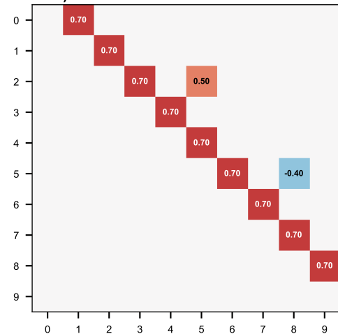
a) Ground truth shared backbone W0
