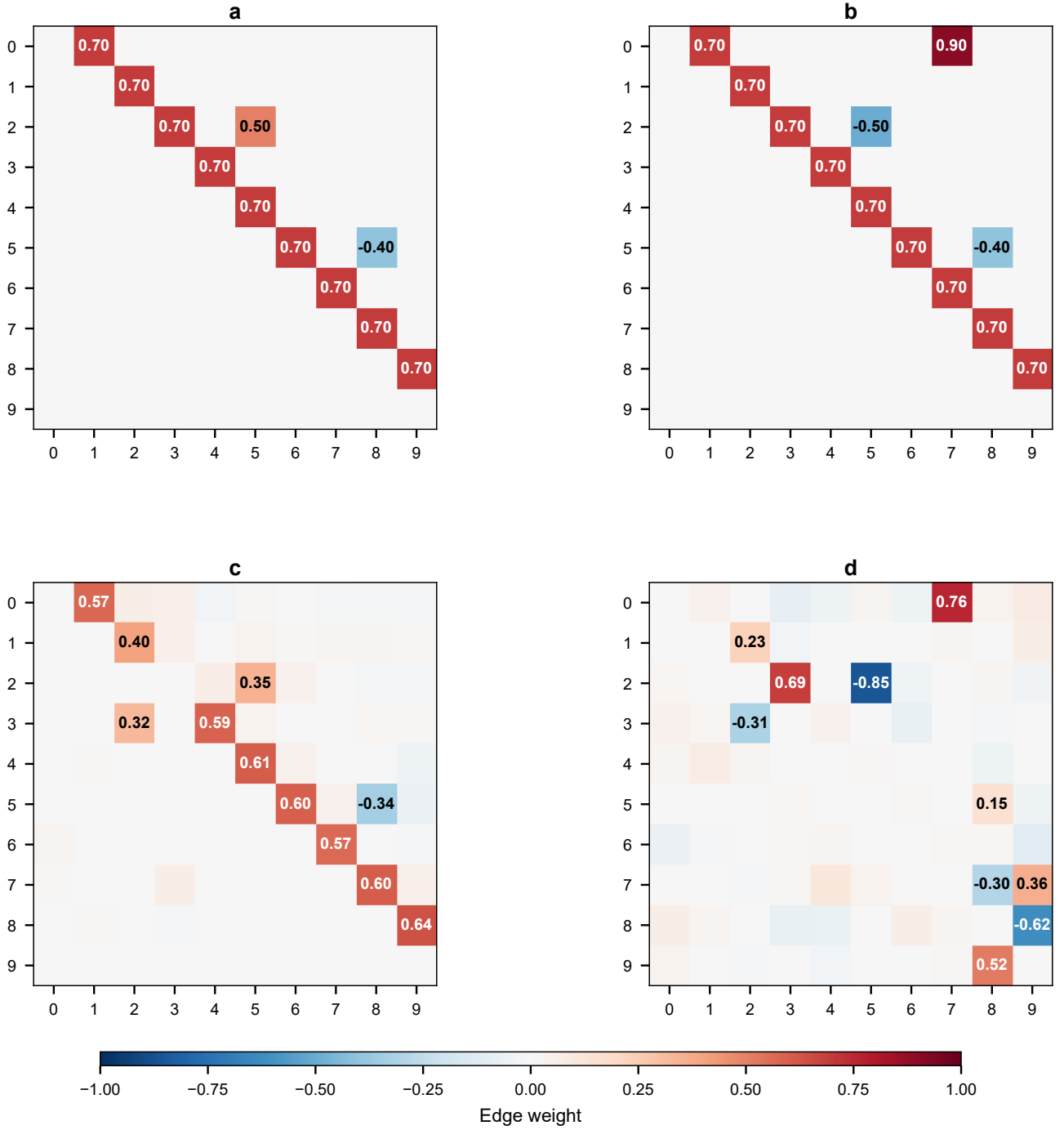
Fig. S2 Two-stage decomposition validation on a synthetic Erdős-Rényi DAG ( d = 10 , K = 3 ). a ) Ground truth shared backbone W_0 (11 edges). b ) Ground truth Batch 1: rewired edge 2 \rightarrow 5 (sign-flipped) and new edge 0 \rightarrow 7 . c ) Recovered \hat{W}_0 from Stage 2 DAG projection (10/11 shared edges above \tau = 0.2 , h(W_0) = 5.21 \times 10^{-6} ). d ) Deviation matrix \Delta_1 = \hat{W}_1 - \hat{W}_0 for the rewired batch. Overall recall: 14/15 ground-truth edges recovered ( = 0.93 ); see Table 2 of the main text for Precision, F1, FDR, and SHD
