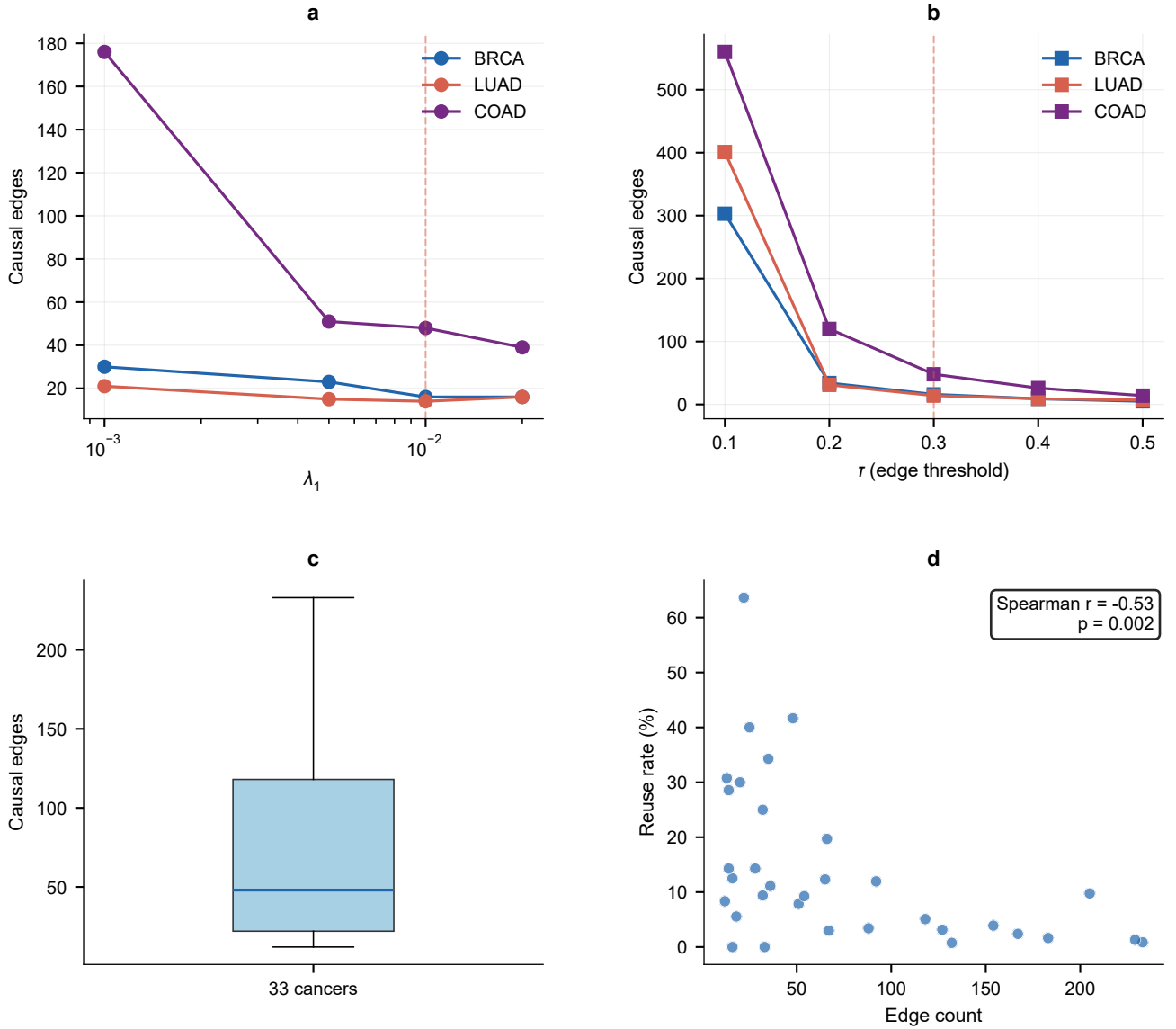
Fig. S1 Parameter sensitivity of the NOTEARS pipeline. a ) \ell_1 regularization sensitivity for three representative cancers; \lambda_1 = 0.01 selected (dashed). b ) Edge threshold \tau sensitivity; \tau = 0.3 selected (dashed). c ) Edge count distribution across 33 cancers (boxplot; mean 74.1, SD 67.7). d ) Edge count vs per-cancer reuse rate (Spearman r = -0.53 , p = 0.002 )
