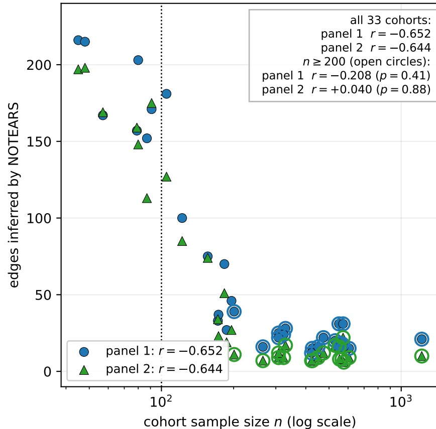
(b) Sample-size dependence reproduces across panels
