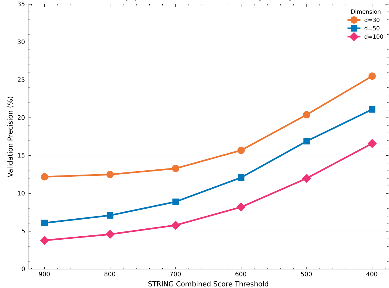
(b) STRING Multi-Threshold (PBMC)
