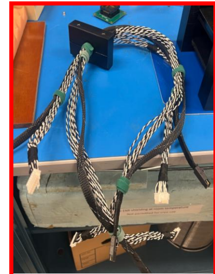
1m Cable Bundle
