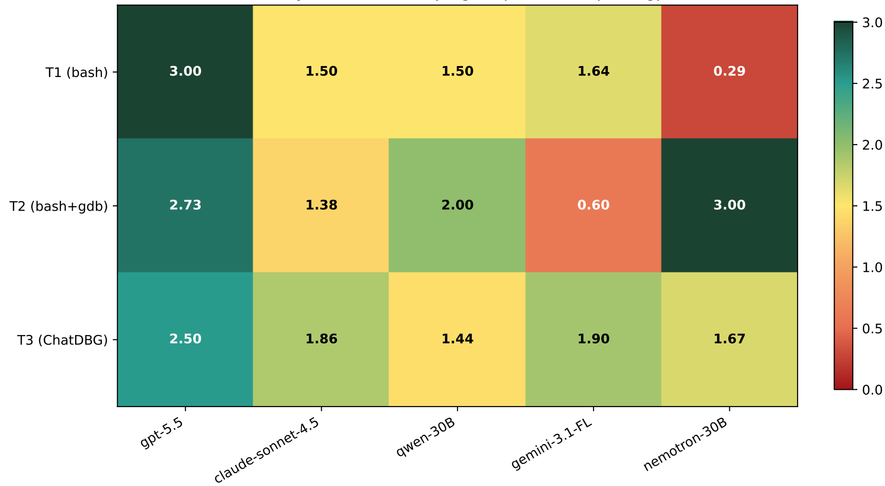
Mean total score (root_cause + local_fix + global_fix, /3) across 4 synthetic cases — judge=openrouter/openai/gpt-4o
