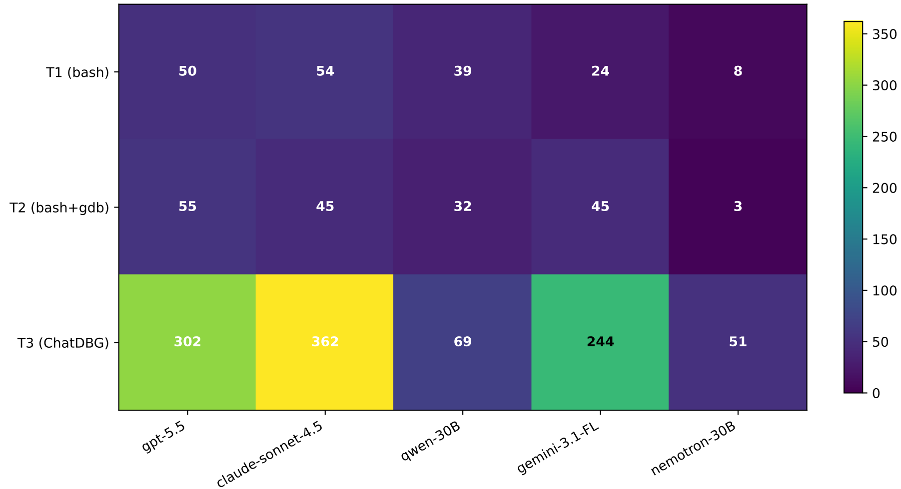
Total tool calls (summed over 4 cases) — agent engagement
