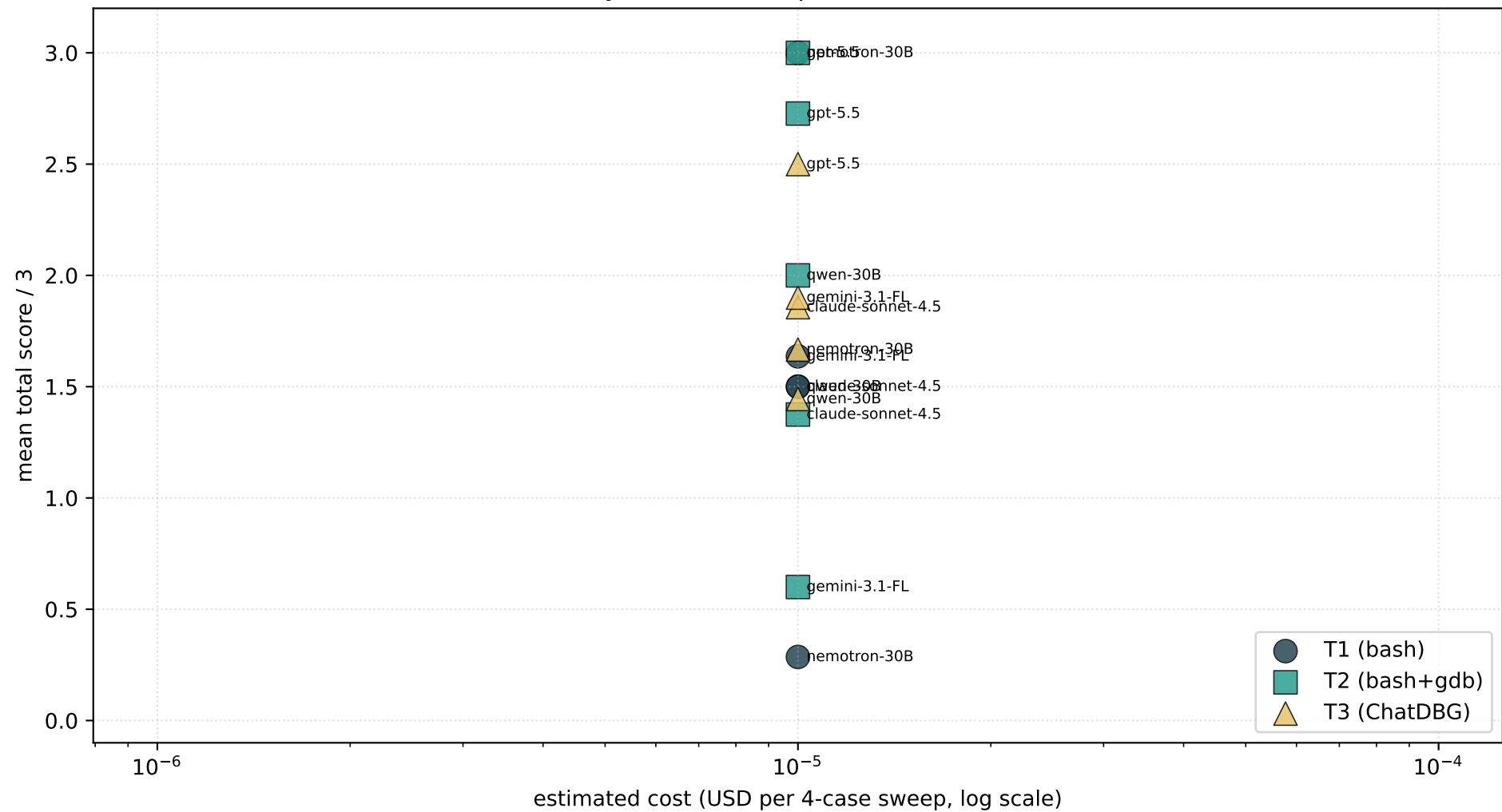
Cost-effectiveness: mean score vs. sweep cost (4 synthetic cases per (tier × model))
