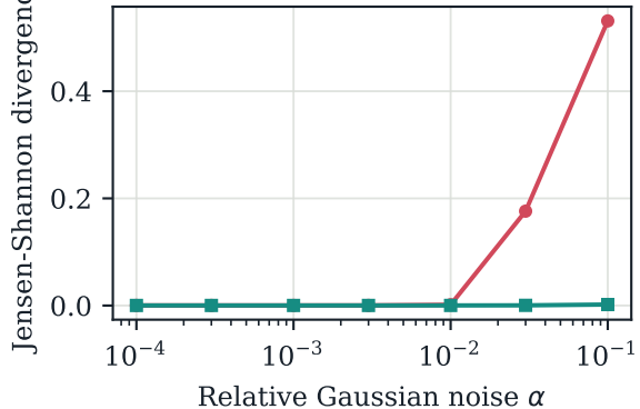
Distribution drift
