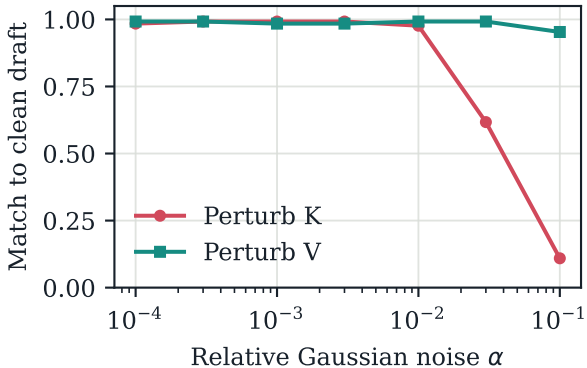
Top-1 stability
