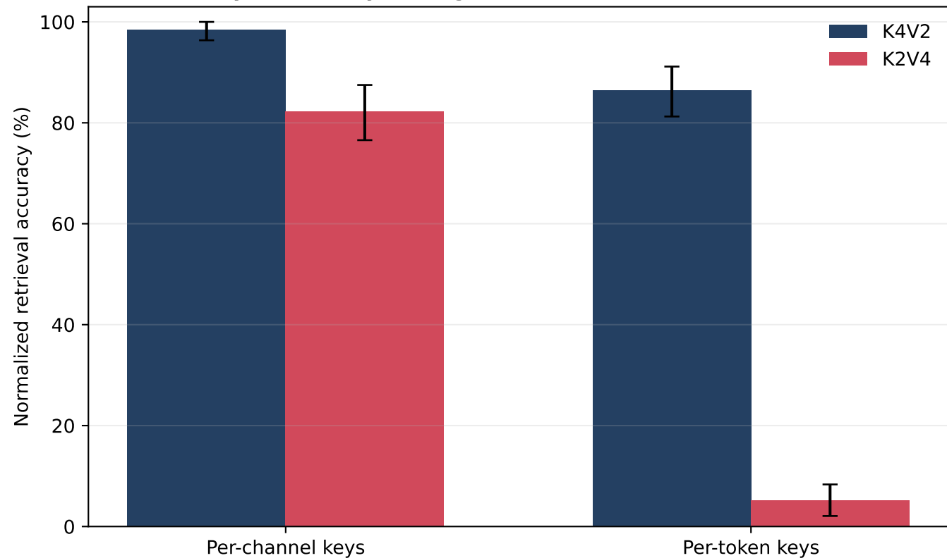
Key Geometry Changes the K/V Precision Tradeoff
