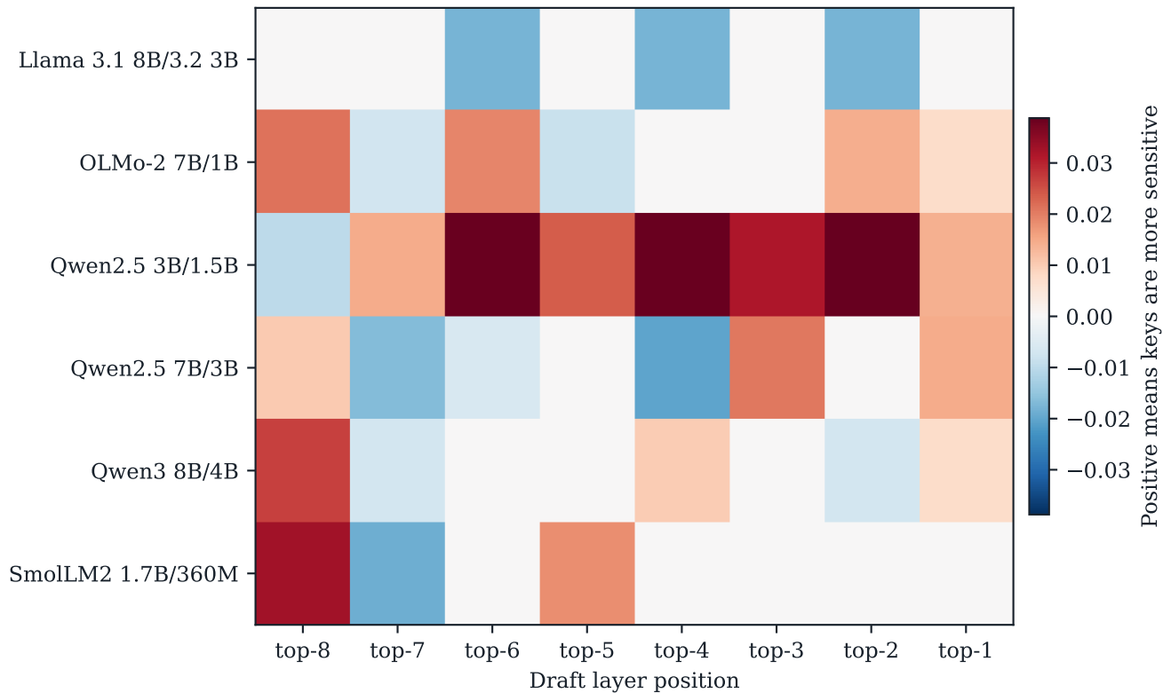
4-bit sensitivity: acceptance drop(K) - drop(V)
