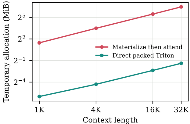
Dequantization workspace
