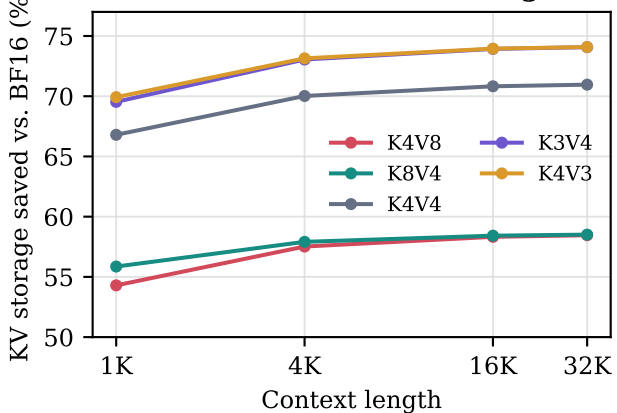
Metadata-inclusive savings
