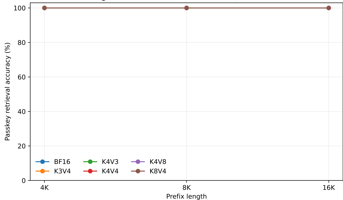
Long-Context Retrieval under KV Quantization
