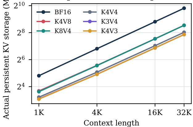
Bit-packed cache footprint
