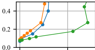
Wan - Ycsb
