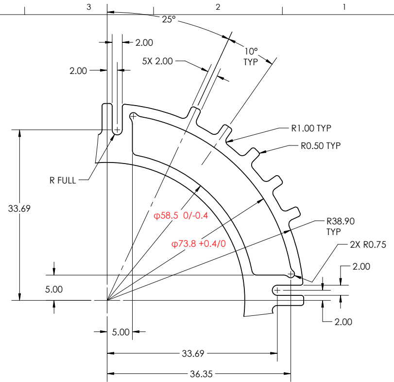
DETAIL A 4PLACES SCALE 2 : 1
