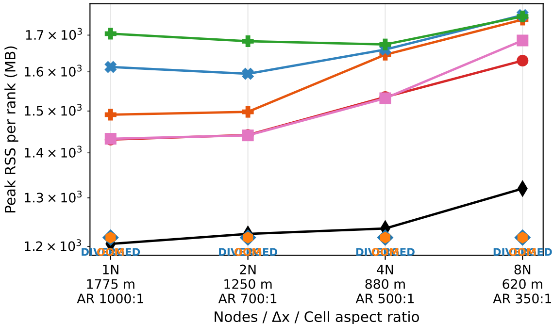
Peak memory per rank
