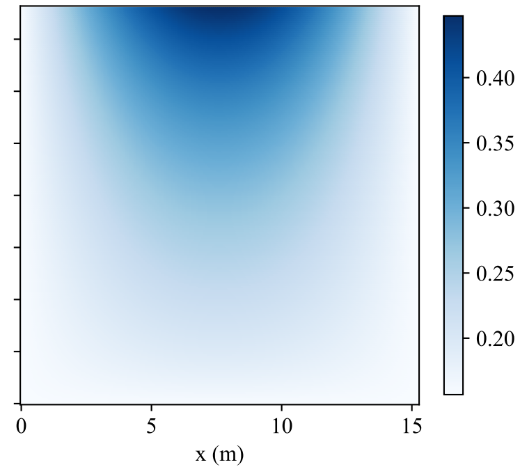
Numerical \theta
