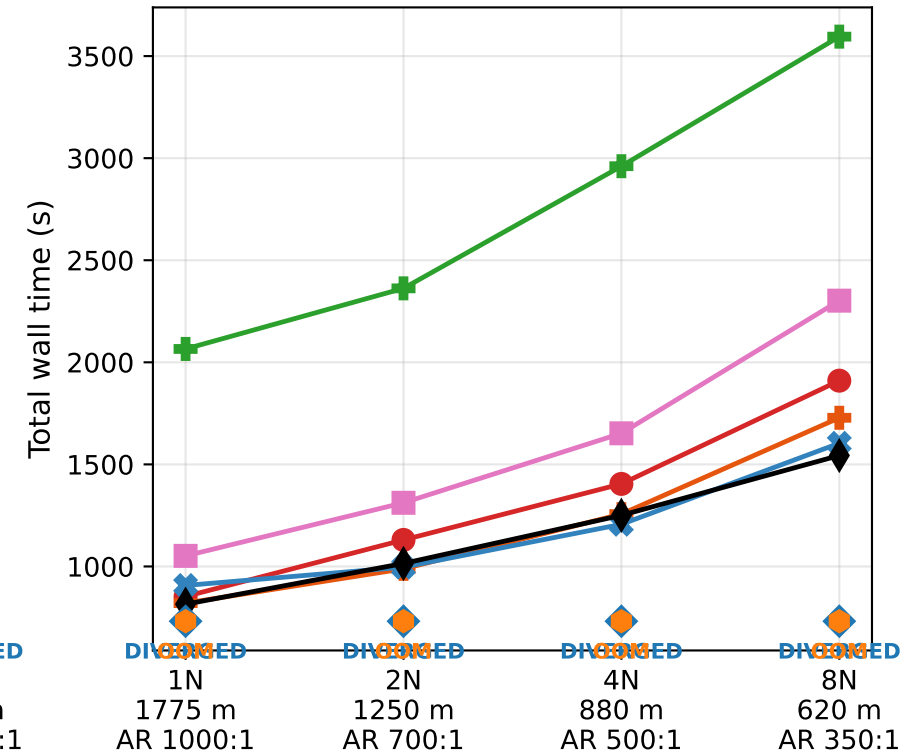
(f) Total wall time
