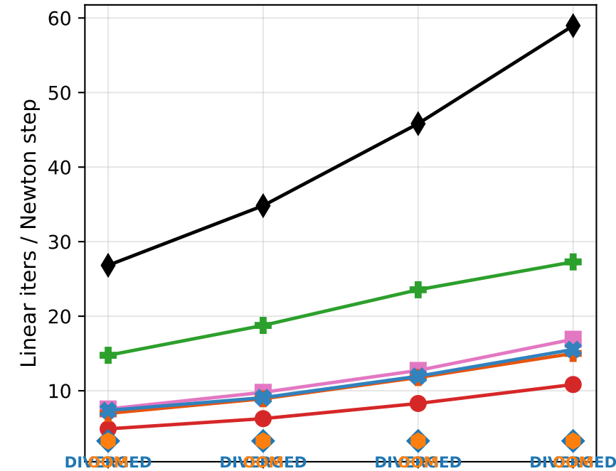
(a) Krylov iters per Newton step
