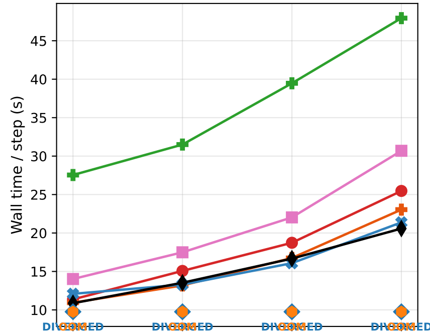
(b) Wall time per step (all)
