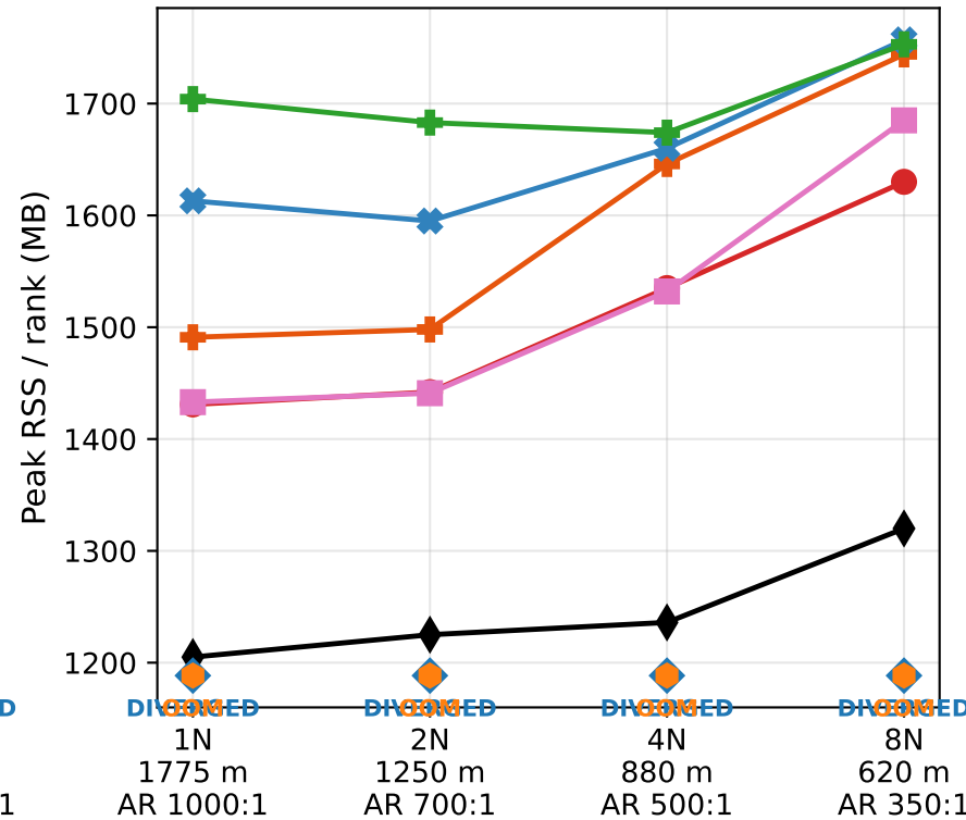
(e) Peak memory per rank
