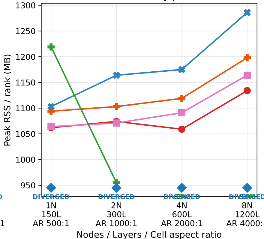
(e) Peak memory per rank
