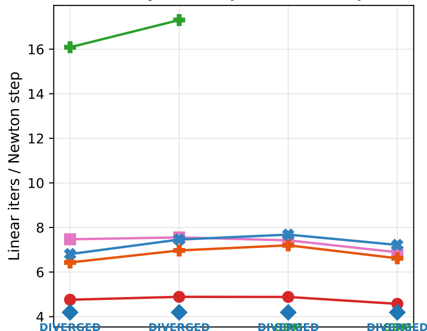
(a) Krylov iters per Newton step
