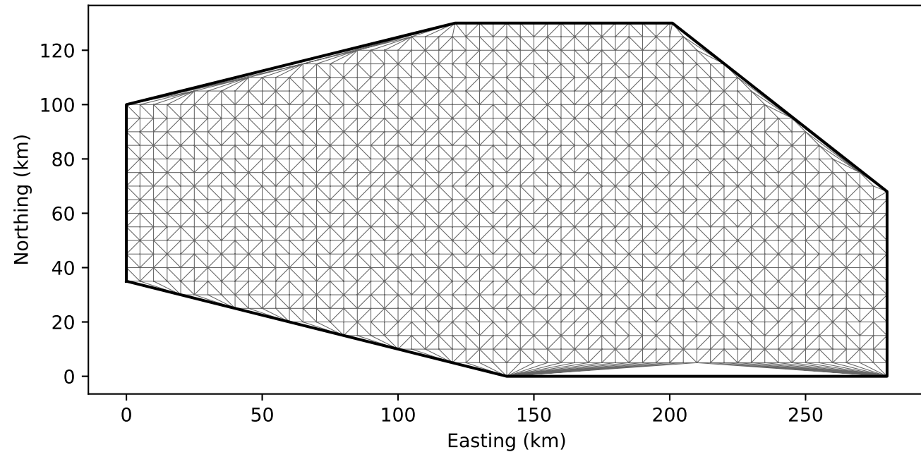
(a) Surface mesh ( \Delta x \approx 5 km)
