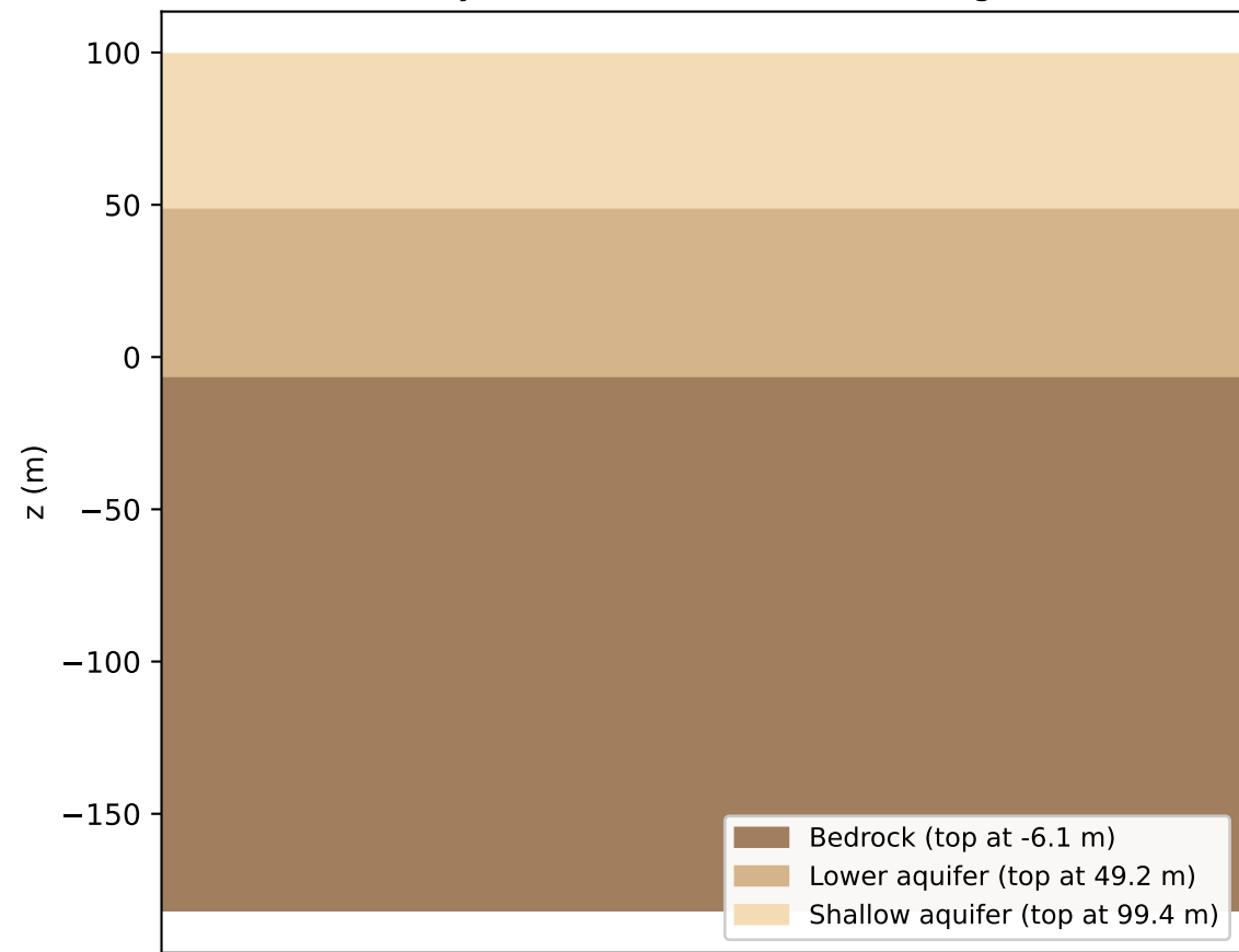
(a) Layer schematic (domain averages)
