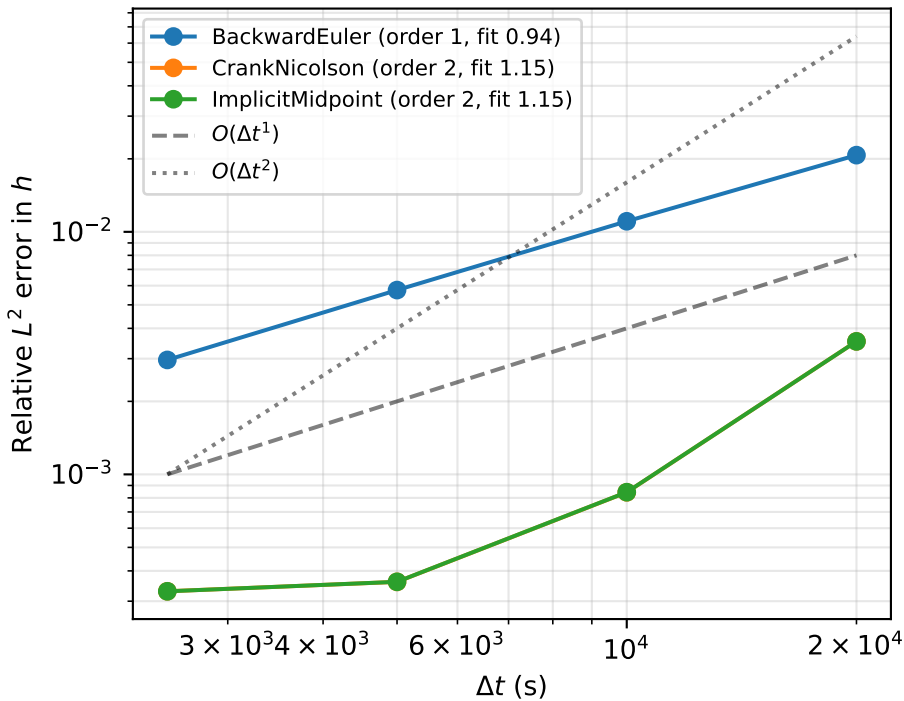
Tracy 2D temporal convergence (DQ1, 201 2 )
