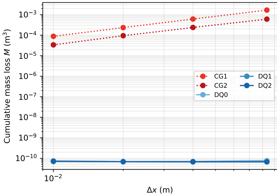
Mass conservation vs \Delta x ( \Delta t = 100 s)
