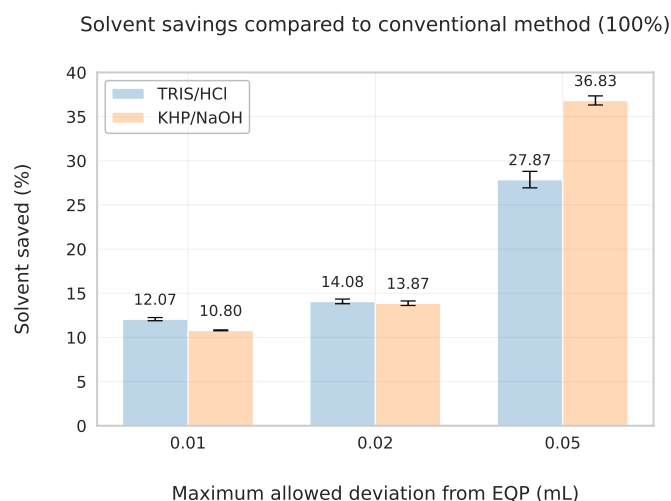
Fig. 2 Solvent savings achieved by stopping at the optimal earliest acceptable point volume using different acceptance criteria (0.01, 0.02 and 0.05 mL difference from the full-dataset EQP). Results are shown for both TRIS/HCl and KHP/NaOH systems ( n = 6 replicates each) and compared against the equivalence point and full titration endpoint
