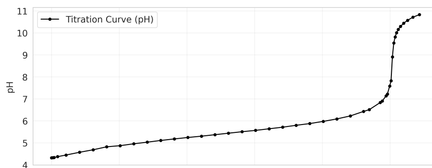
Opt Schwartz EQP = 5.035 mL, k = 0.364
