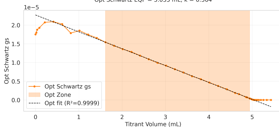
Opt Schwartz EQP = 5.035 mL, k = 0.364
