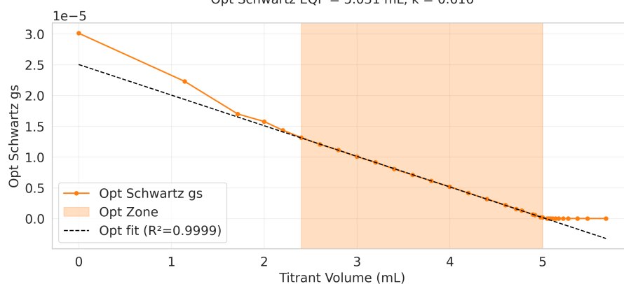
Opt Schwartz EQP = 5.031 mL, k = 0.616
