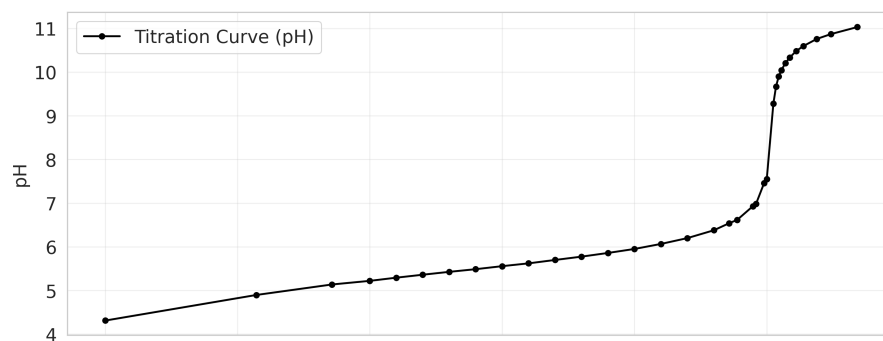
Opt Schwartz EQP = 5.031 mL, k = 0.616
