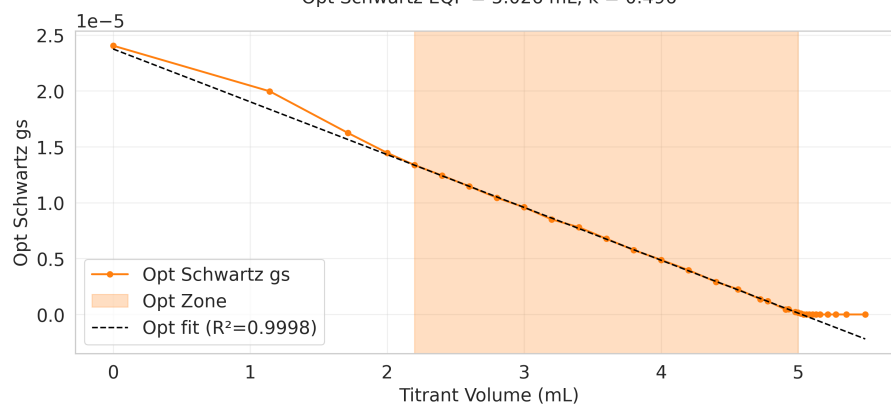
Opt Schwartz EQP = 5.026 mL, k = 0.496
