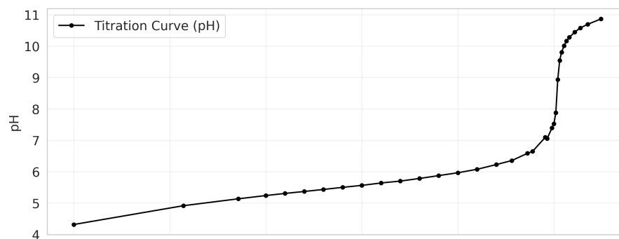
Opt Schwartz EQP = 5.026 mL, k = 0.496
