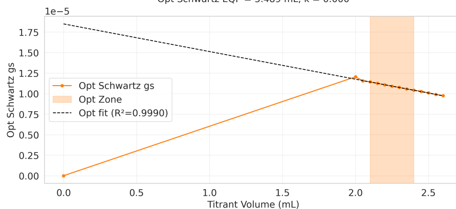
Opt Schwartz EQP = 5.489 mL, k = 0.000
